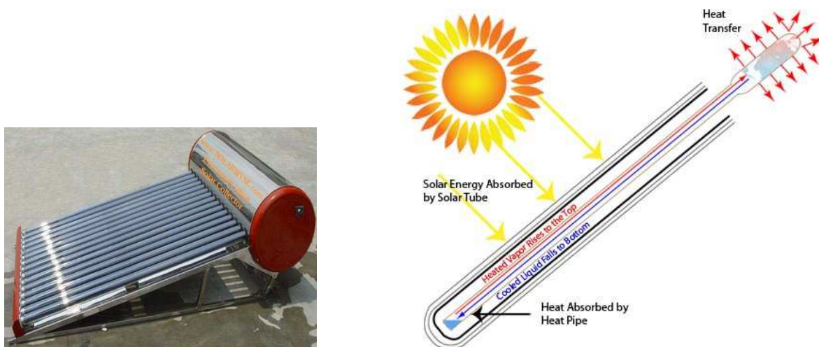
FIGURE 4 - An evacuated-tube SWH
